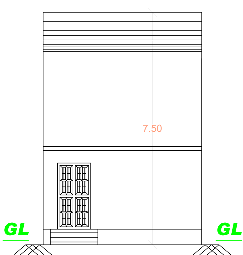
FRONT ELEVATION
