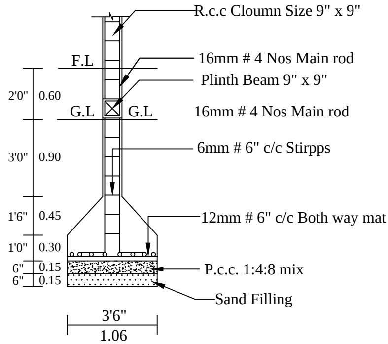
COLUMN DETIALS
