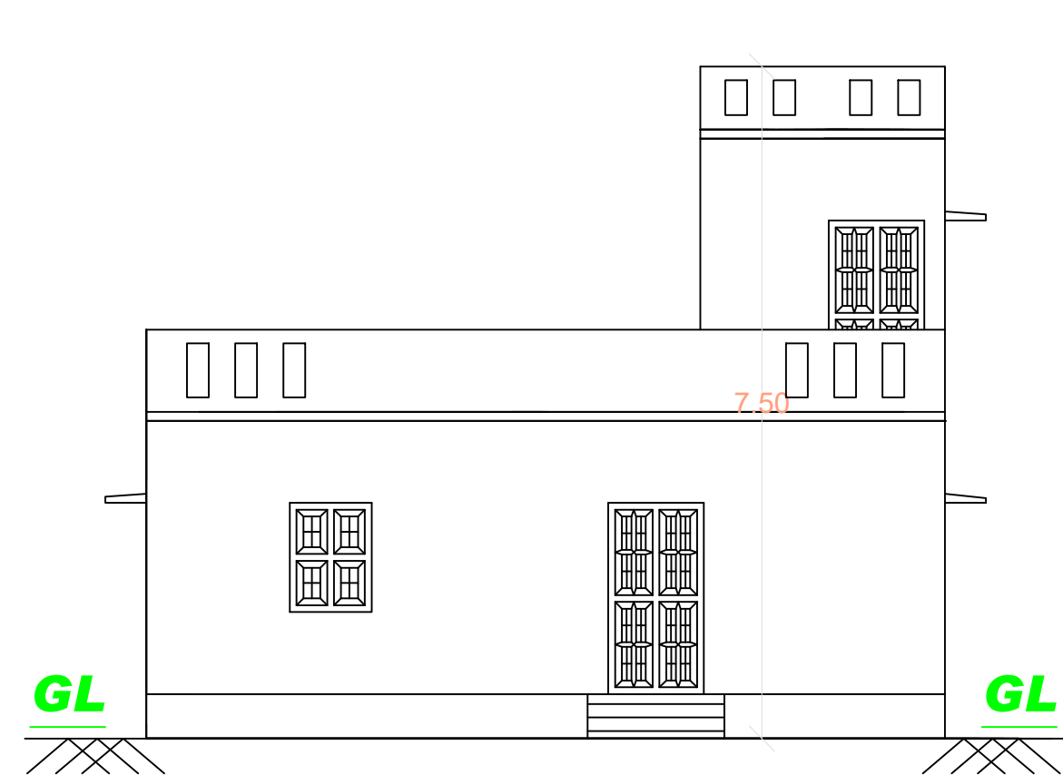
FRONT ELEVATION
