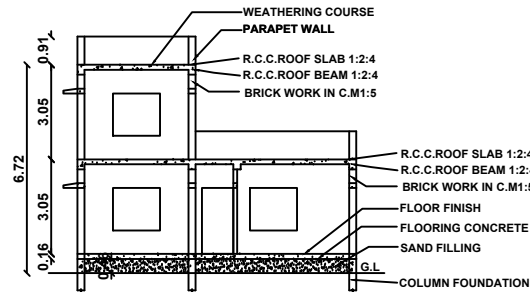
SECTION ON GG
