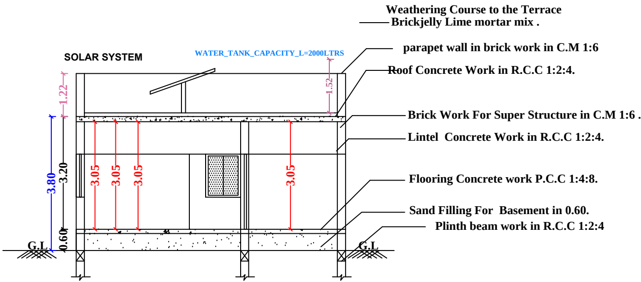
SECTION-AB
