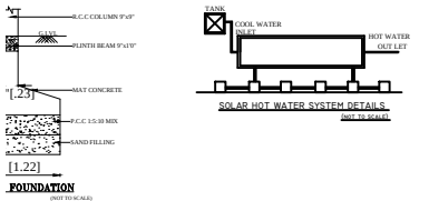
SOLAR HOT WATER SYSTEM DETAILS
