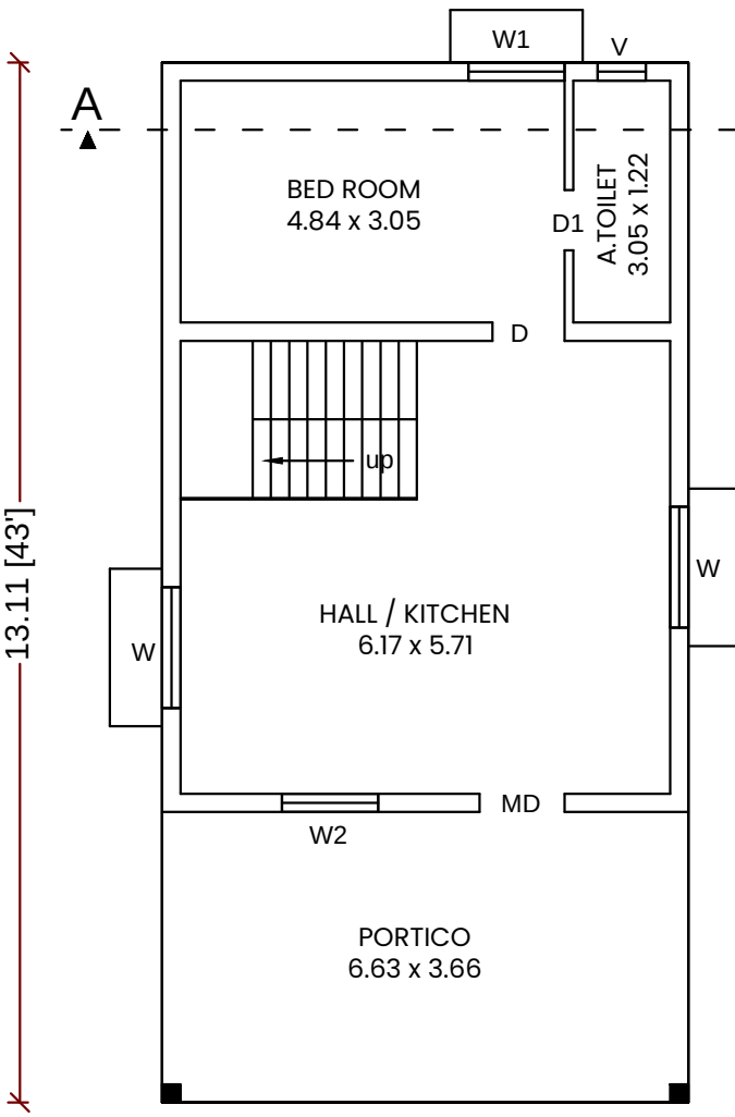
PLAN
