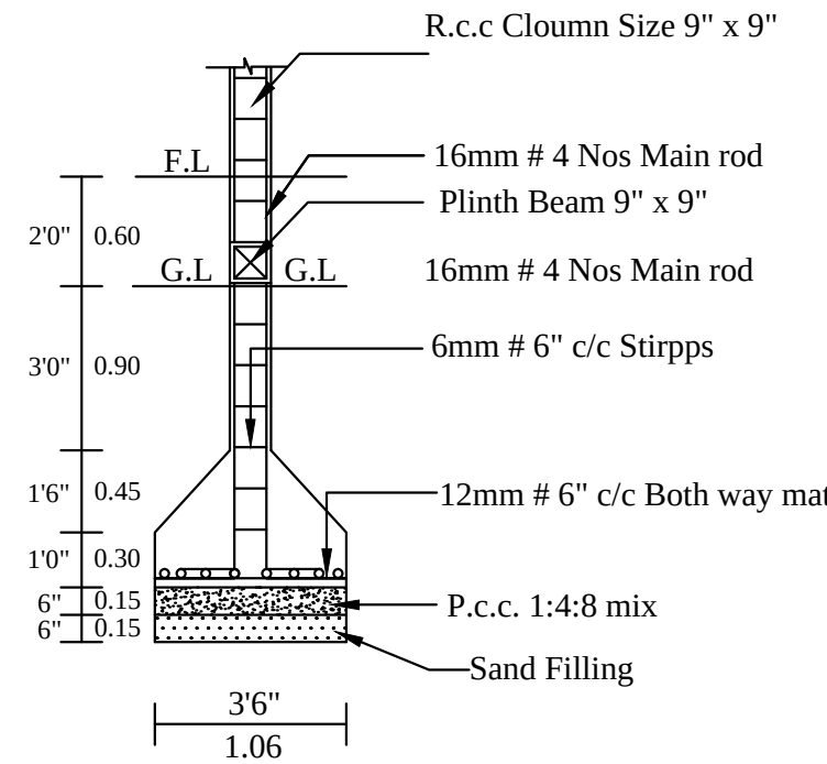
COLUMN DETAILS
