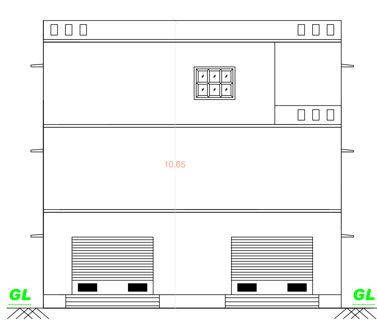
FRONT ELEVATION
