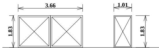
MAIN GATE
