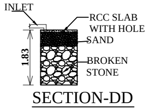
SECTION-DD
