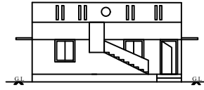
FRONT ELEVATION
