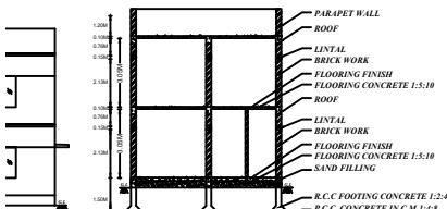
SECTION - BB BLOCK - 2
