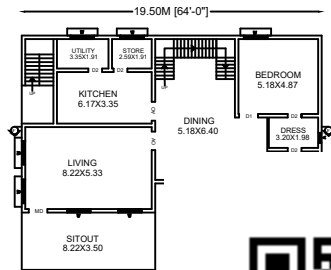
GROUND FL BLOCK
