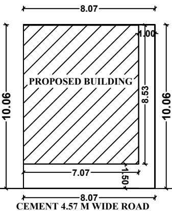
SITE PLAN
