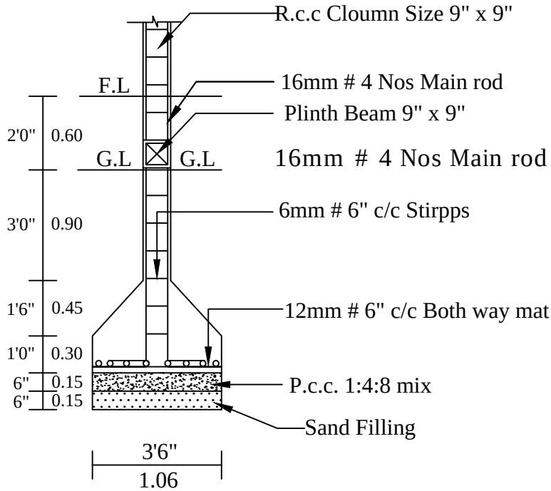
COLUMN DETIAL
