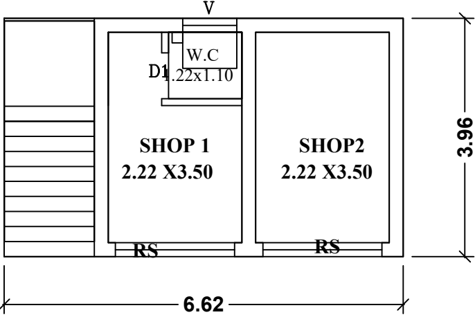
PRO.GROUND FLOOR PLAN
