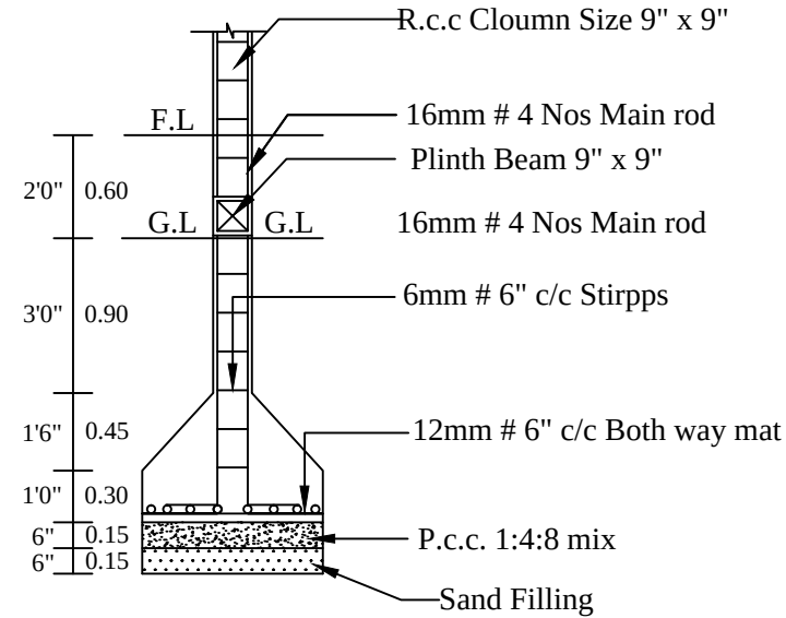
COLUMN DETAILS
