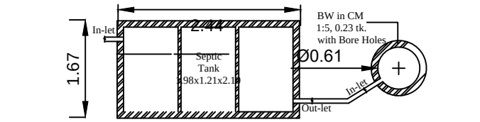
PLAN - SEPTIC TANK & SOAK PIT
