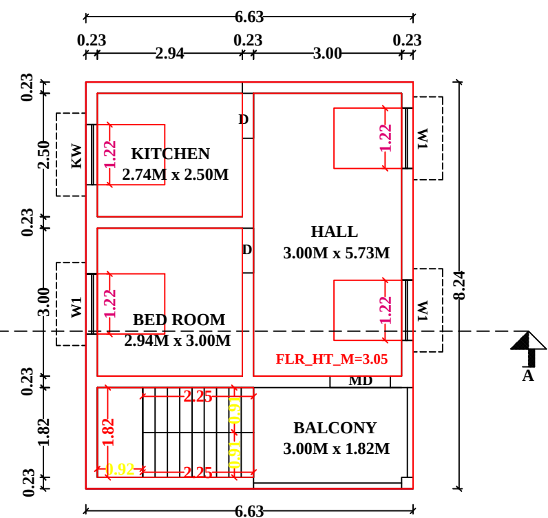
FLOOR-1 PRO.FIRST FLOOR PLAN
