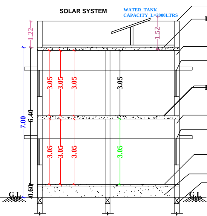
SECTION-AB
