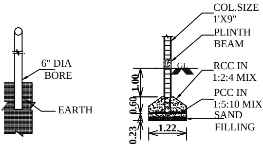
BORE WELL COLUMN DETAILS
