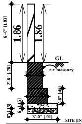
COMPOUND WALL
