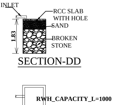
PLAN OF RWH
