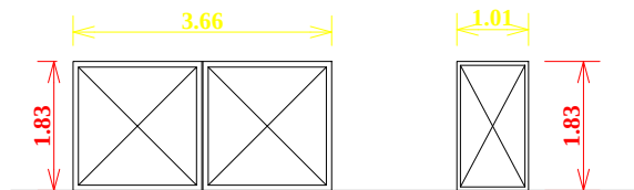
MAIN GATE
