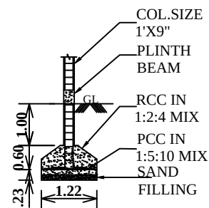
COLUMN DETAILS
