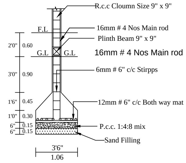
COLUMN DETIAL
