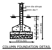
COLUMN FOUNDATION DETAIL
