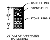
DETAILS OF RAIN WATER HARVESTING
