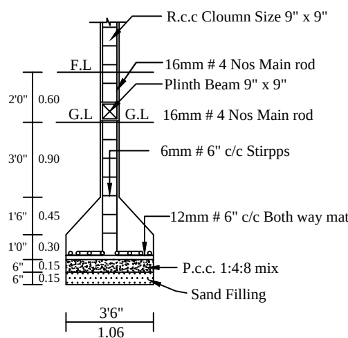
COLUMN DETIALS
