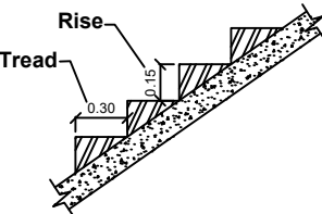
STAIRCASE DETAILS
