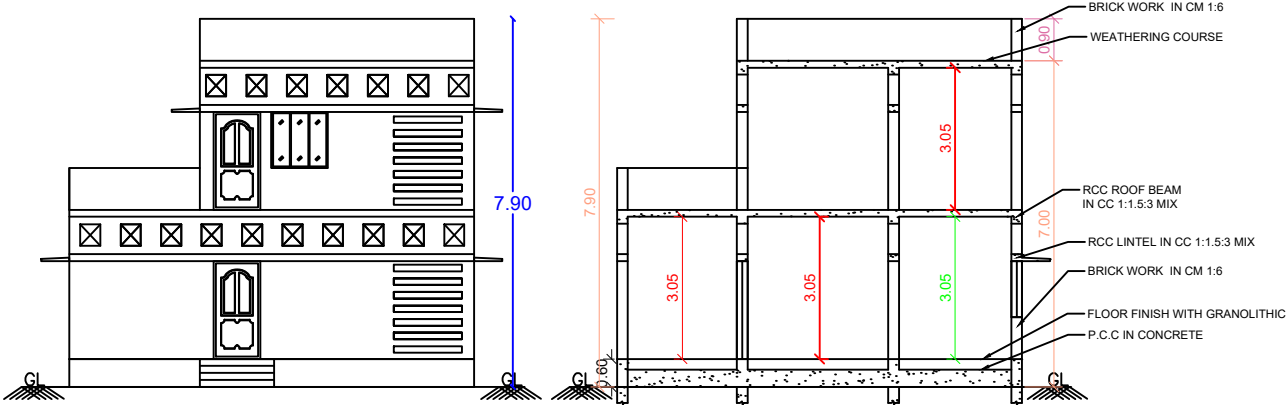
FRONT ELEVATION
