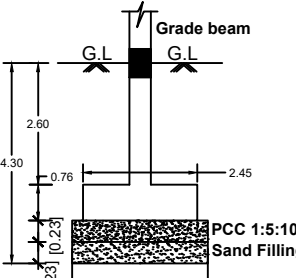
FOUNDATION DETAILS
