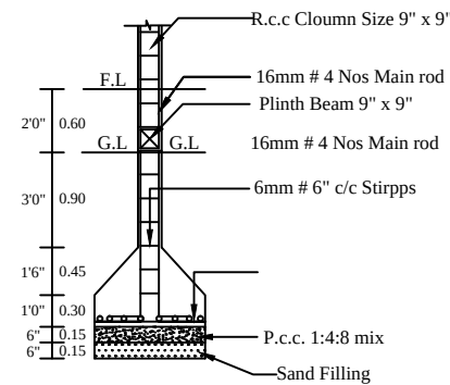
COLUMN DETIALS
