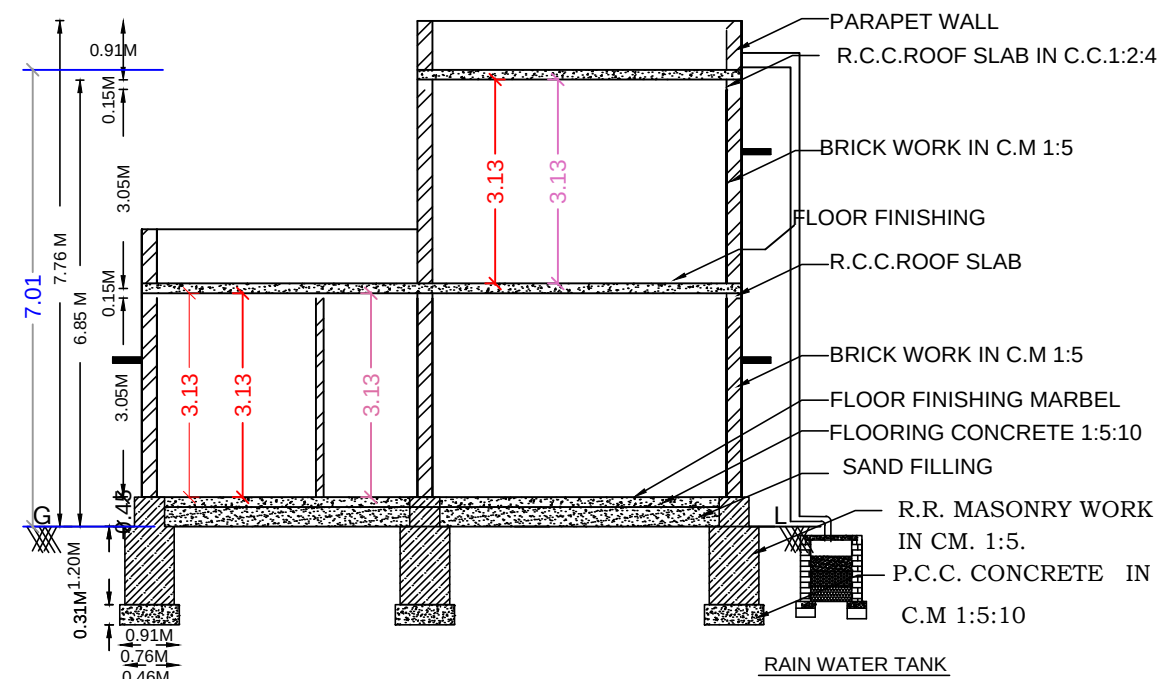
SECTION - XX
