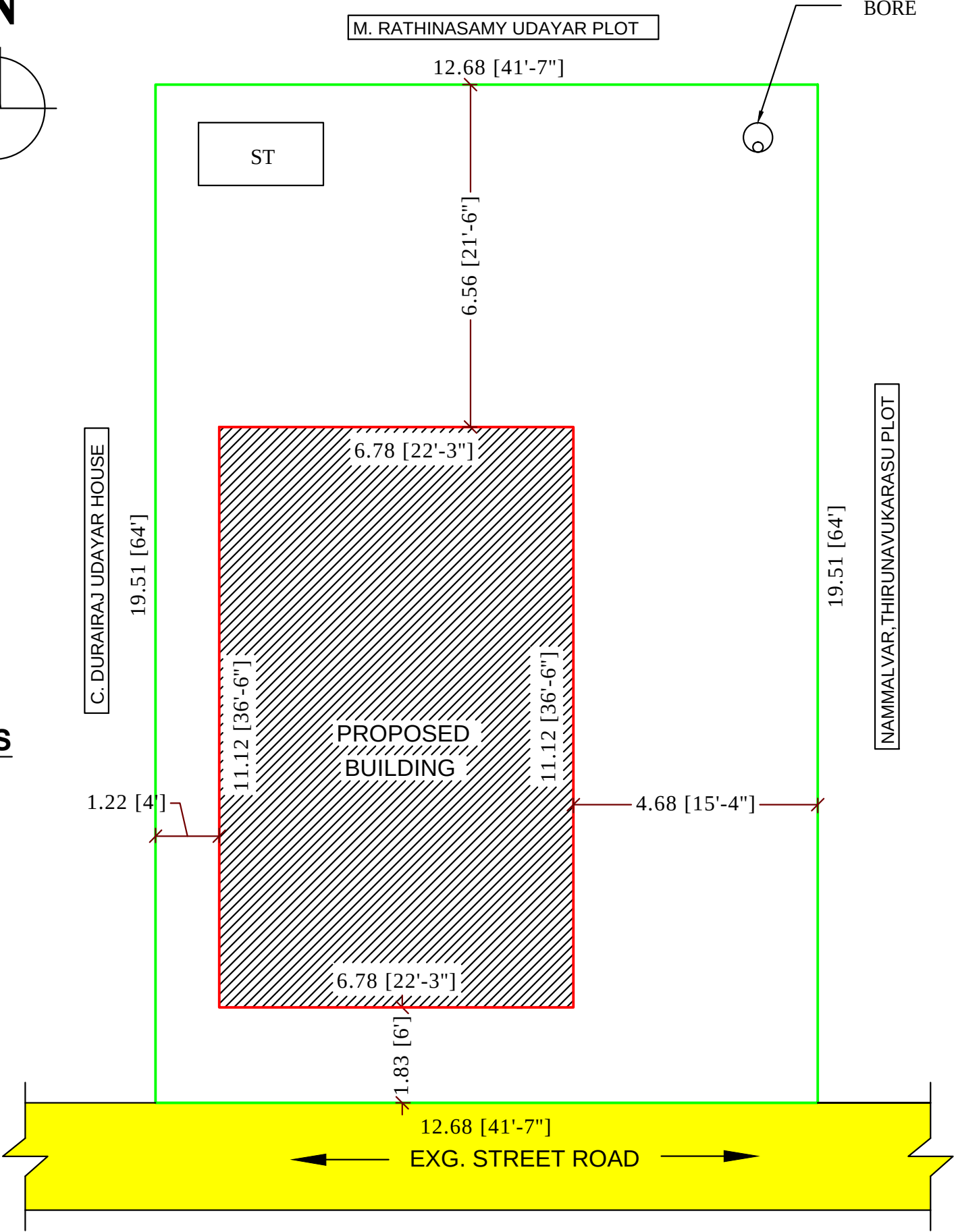
SITE PLAN
