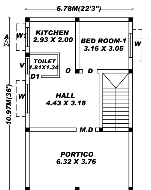
EXG.GROUND FLOOR PLAN
