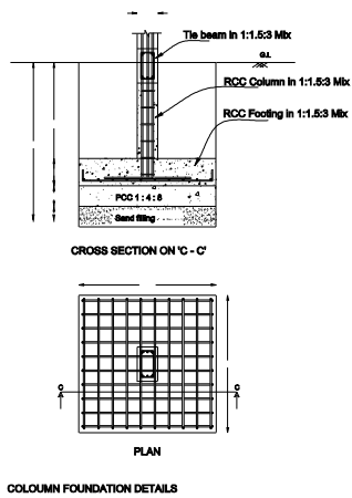
CROSS SECTION ON 'C-C'
