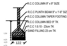
SECTION
