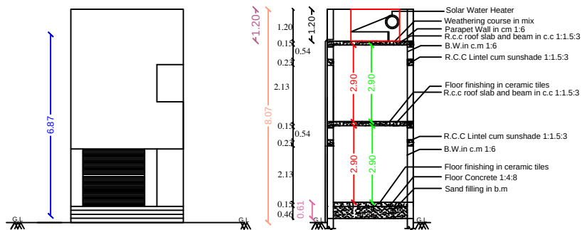
SECTION - "AB - CD "
