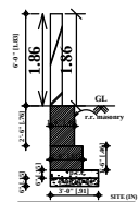
COMPOUND WALL
