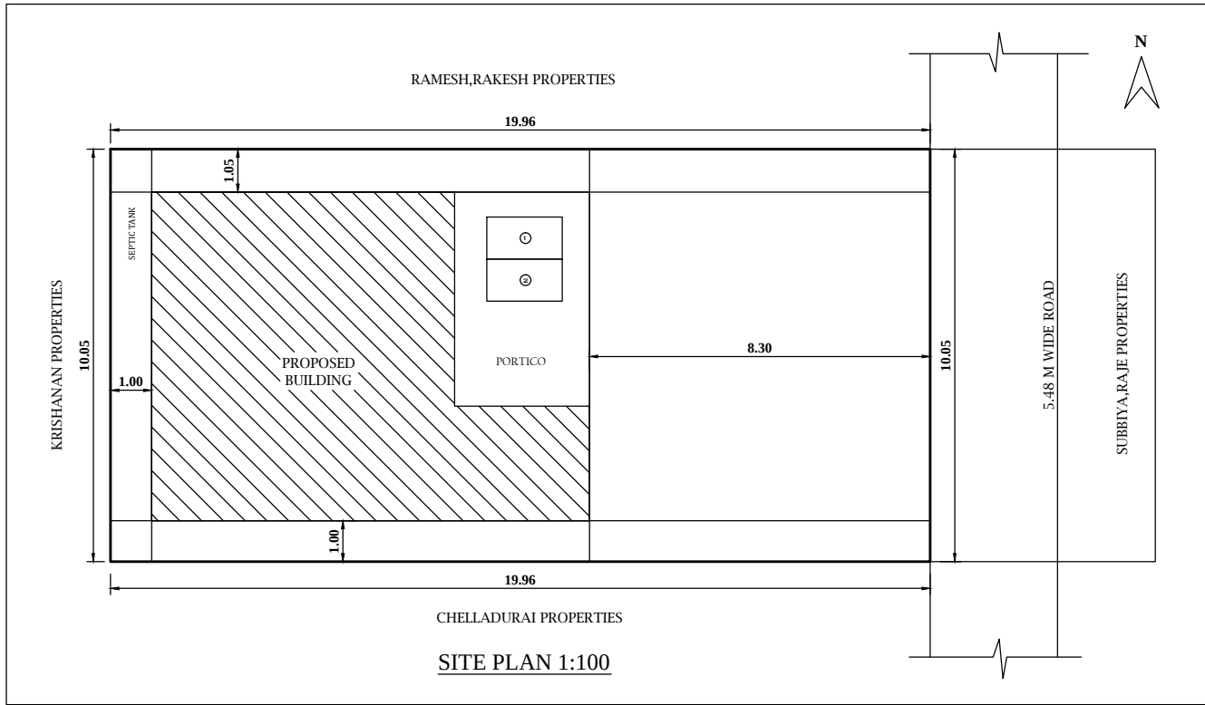
GROUND FLOOR ROOF PLAN
