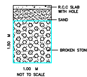
RAIN WATER HARVEST COLLECTION PIT.
