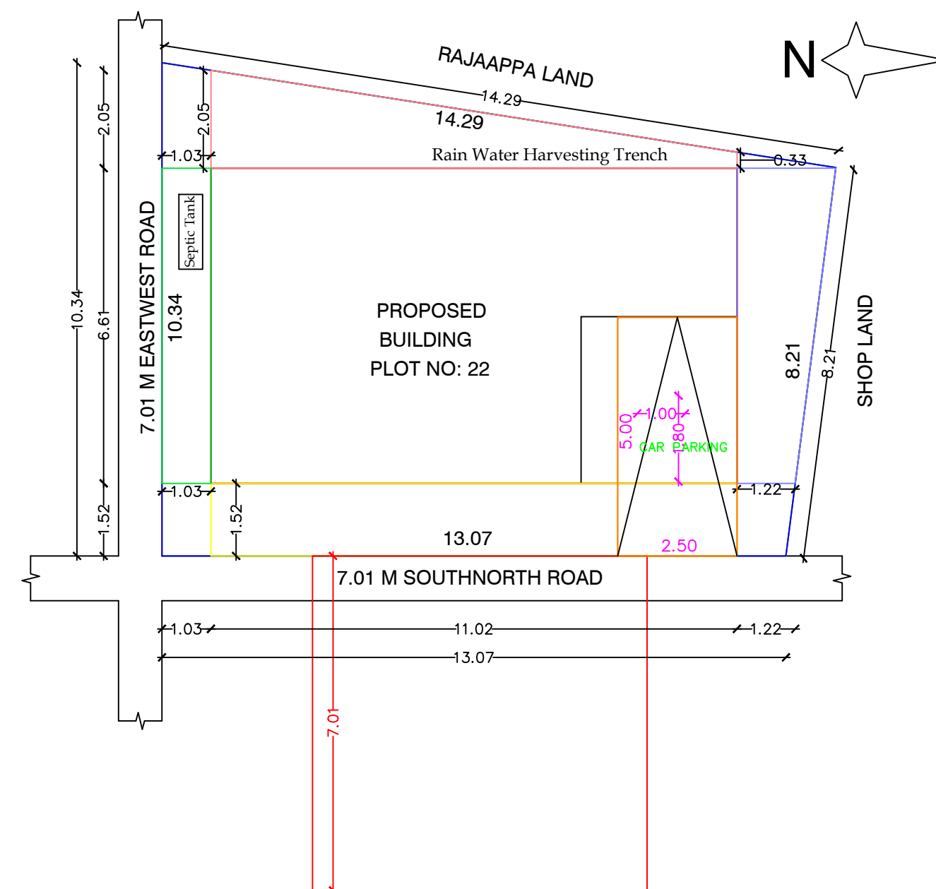
SITE PLAN
