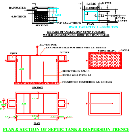
PLAN & SECTION OF SEPTIC TANK & DISPERSION TRENCH
