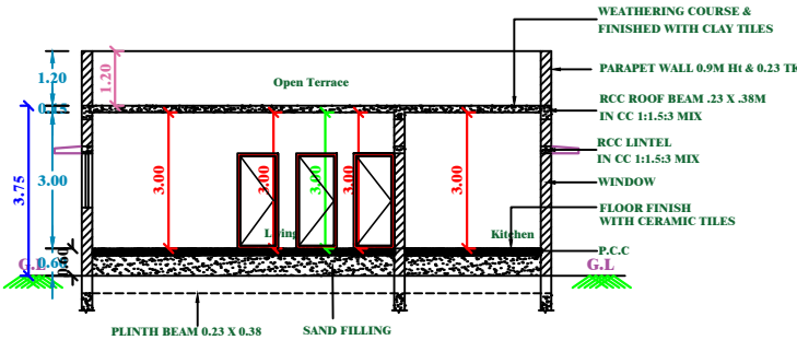
SECTION-XX
