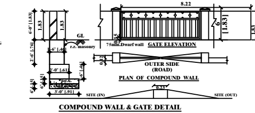
COMPOUND WALL & GATE DETAIL
