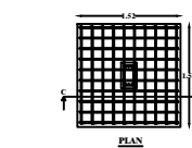
COLOUMN FOUNDATION DETAILS
