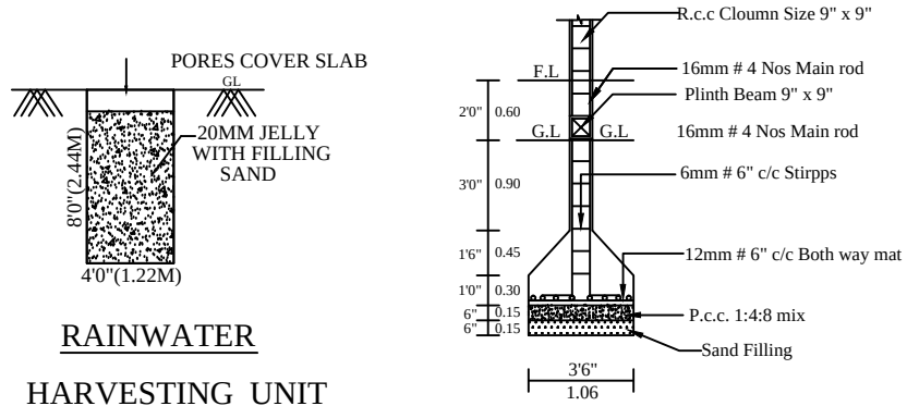
COLUMN DETIAL
