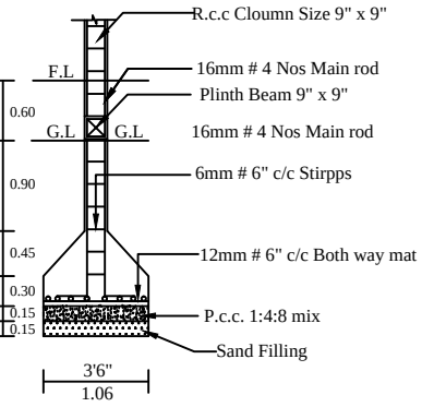
COLUMN DETIAL
