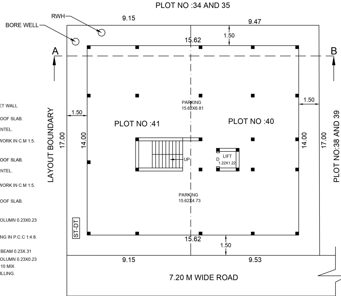
STILT FLOOR CUM SITE PLAN SCALE 1:100.
