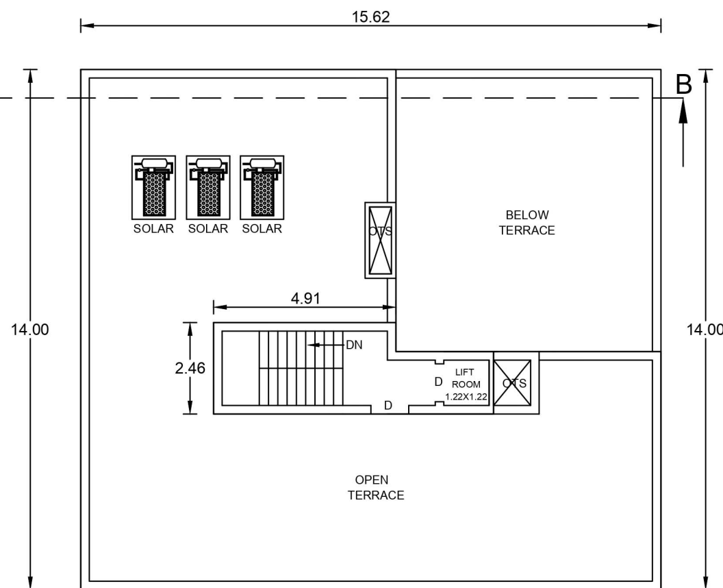
TERRACE FLOOR
