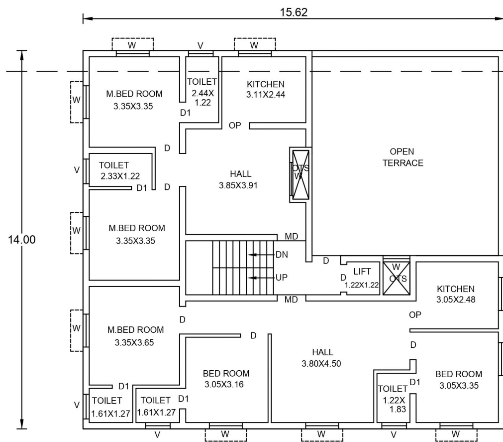
THIRD FLOOR
