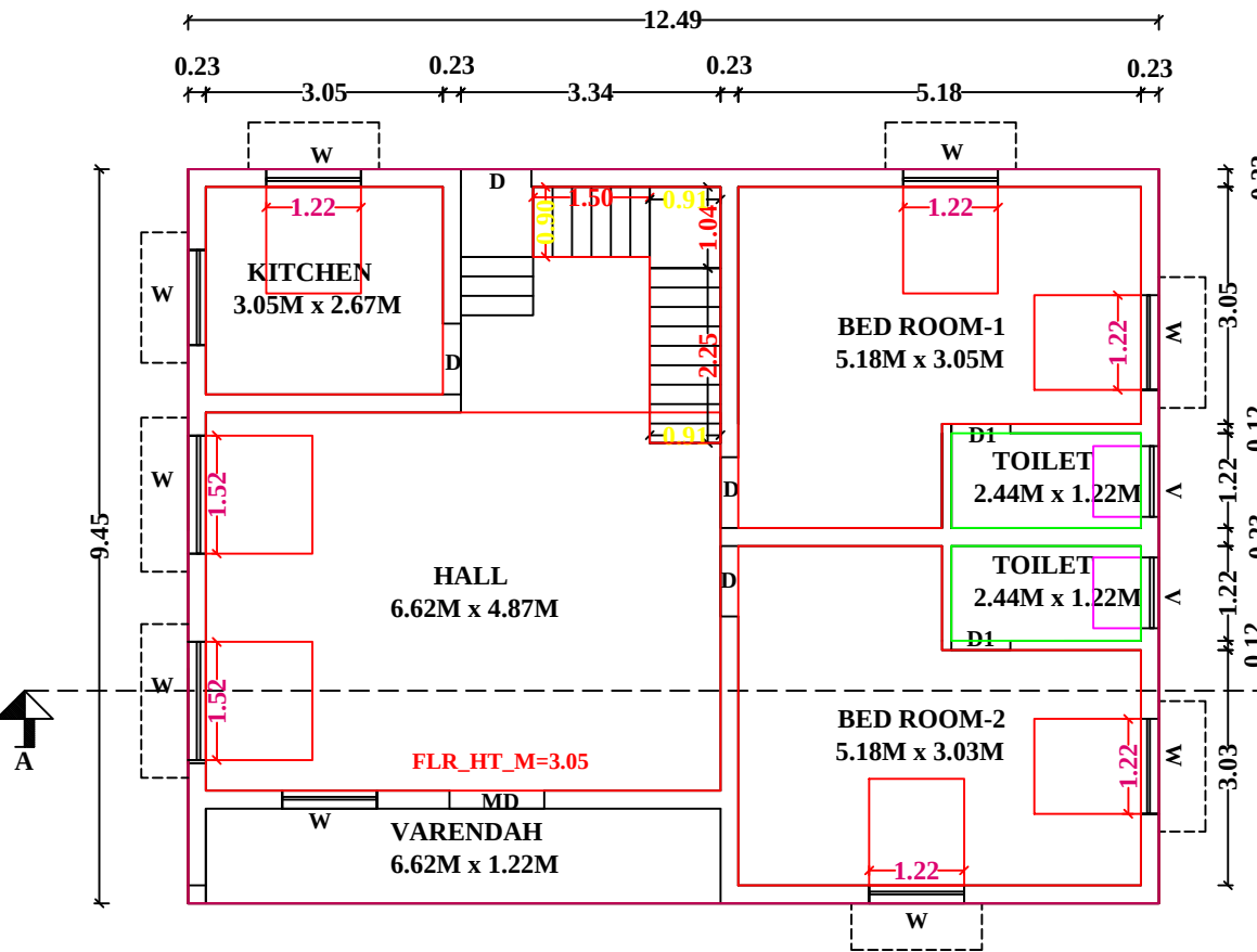
FLOOR-0 PRO.GROUND FLOOR PLAN
