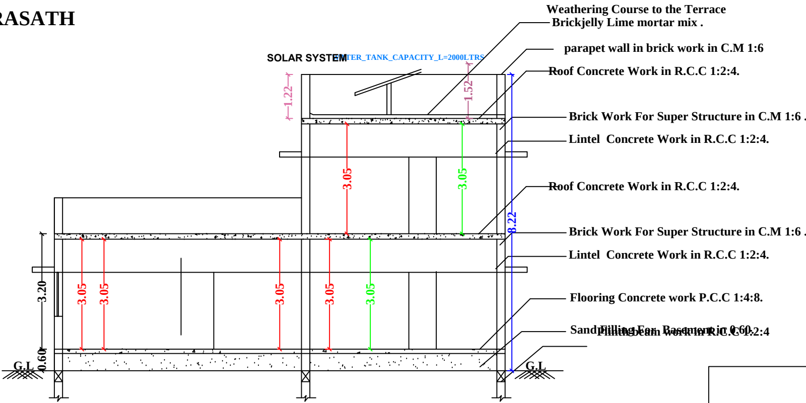
SECTION-AB
