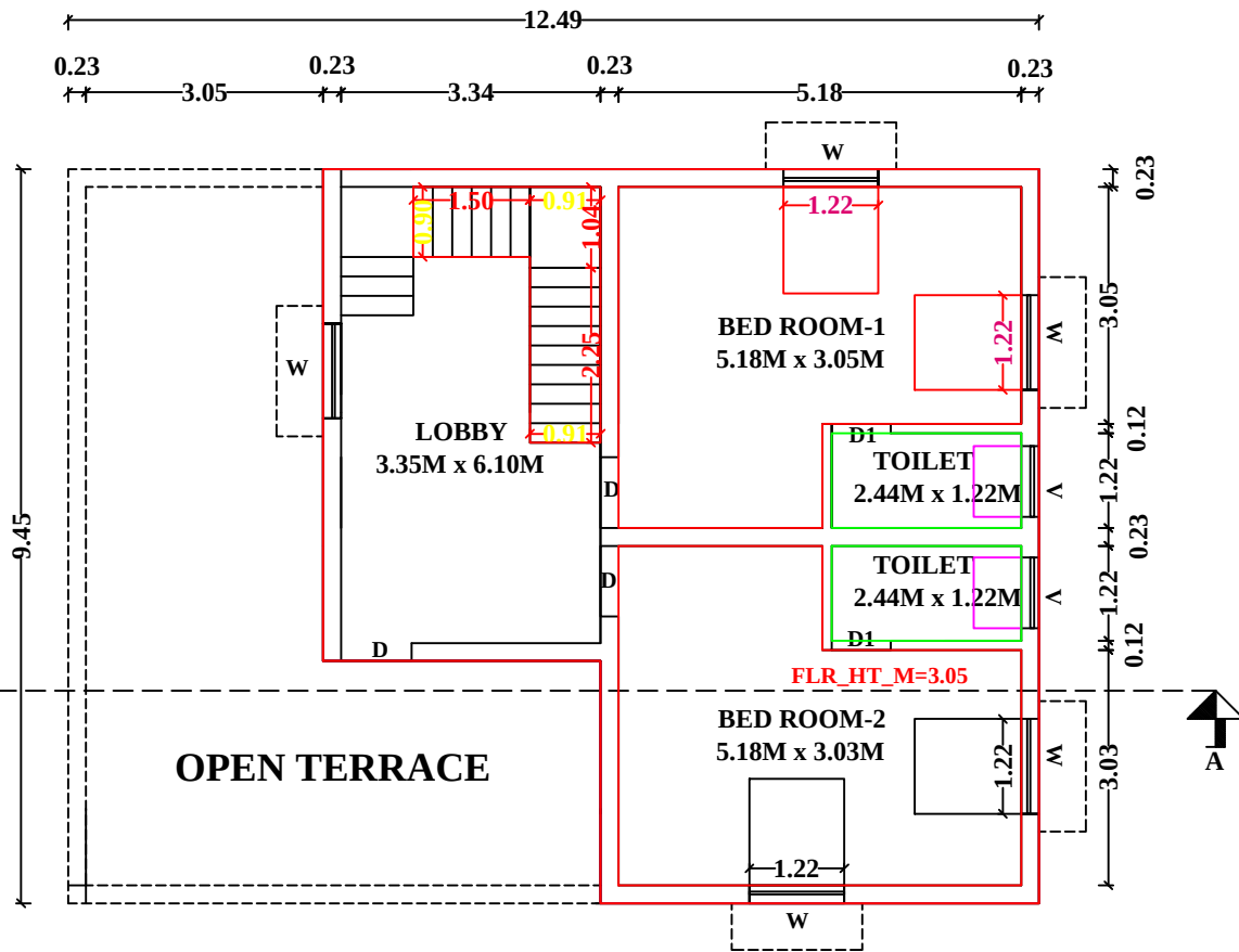
FLOOR-1 PRO.FIRST FLOOR PLAN
