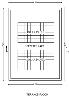
TERRACE FLOOR
