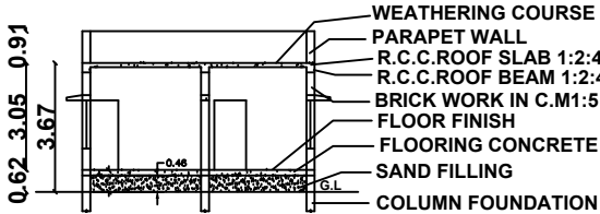
SECTION- SS
