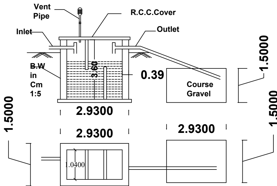
SEPTIC TANK & D-TRENCH DETAILS
