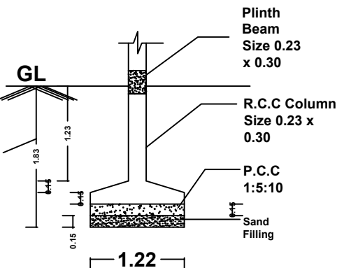
FOUNDATION DETAILS
