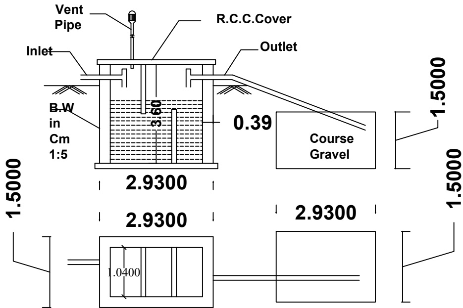
SEPTIC TANK & D-TRENCH DETAILS
