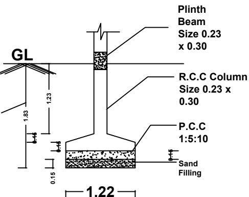
FOUNDATION DETAILS
