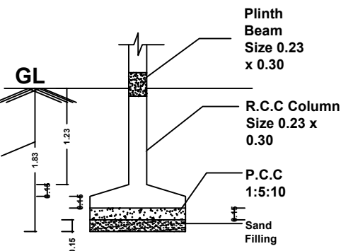
FOUNDATION DETAILS
