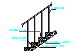
STAIRCASE SECTION
