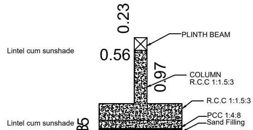
Foundation details
