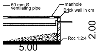
SEPTIC TANK C/S
