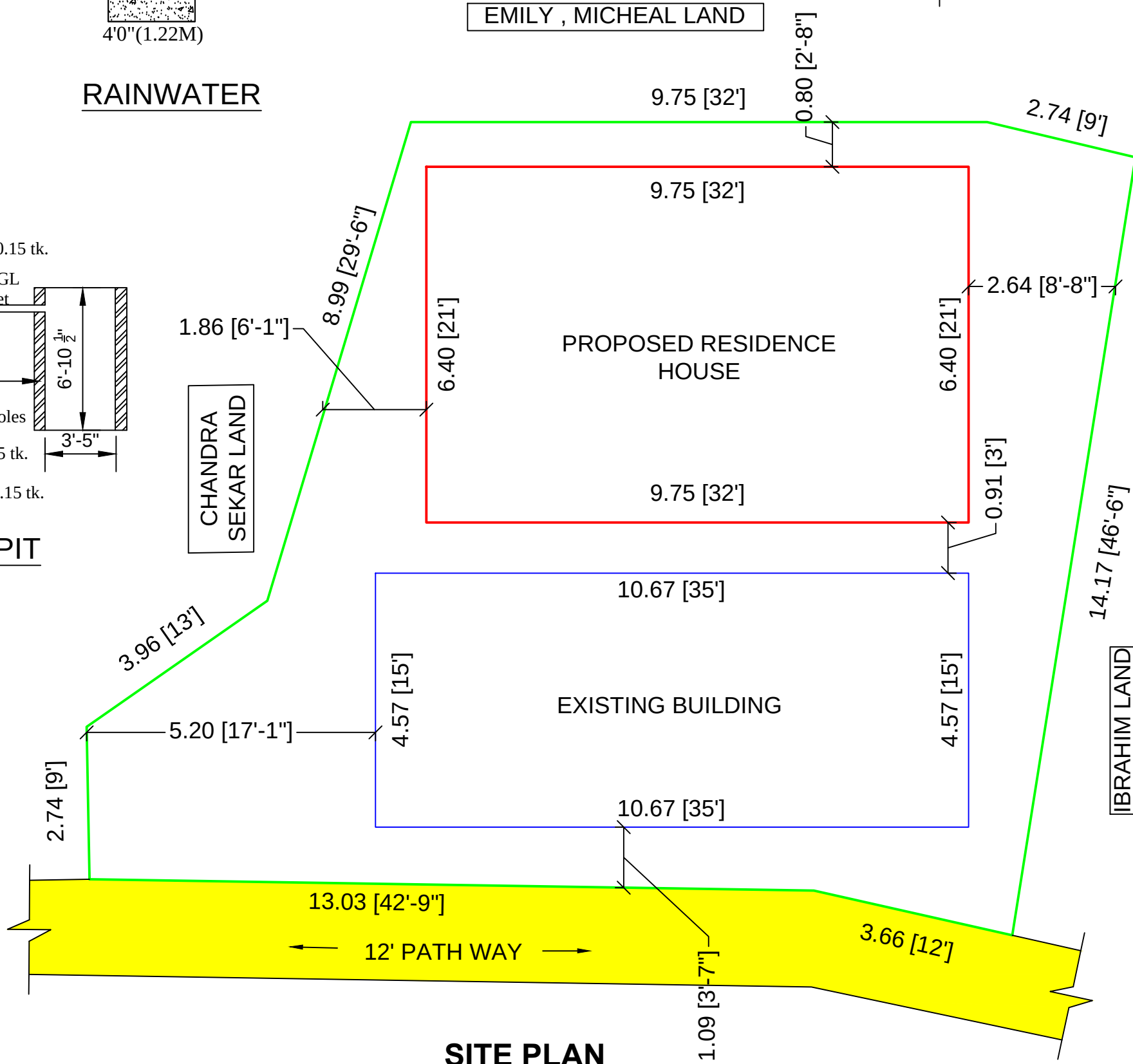
SITE PLAN
