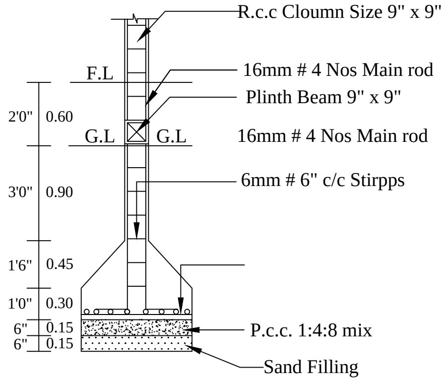
COLUMN DETIALS
