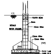
FOUNDATION DETAILS
