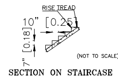
SECTION ON STAIRCASE
