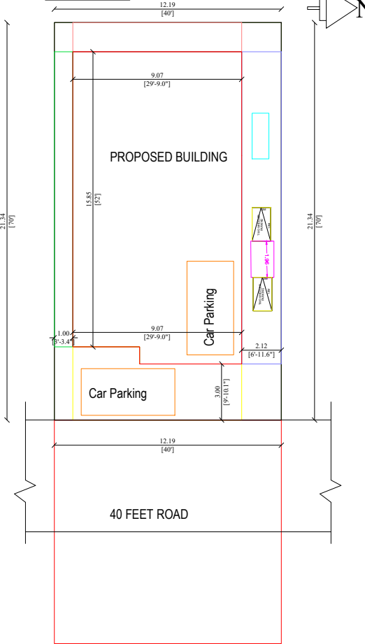
SITE PLAN
