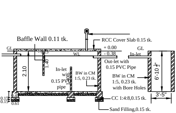
SECTION - SEPTIC TANK & SOAK PIT
