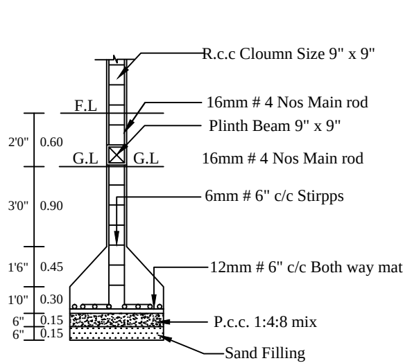
COLUMN DETAILS
