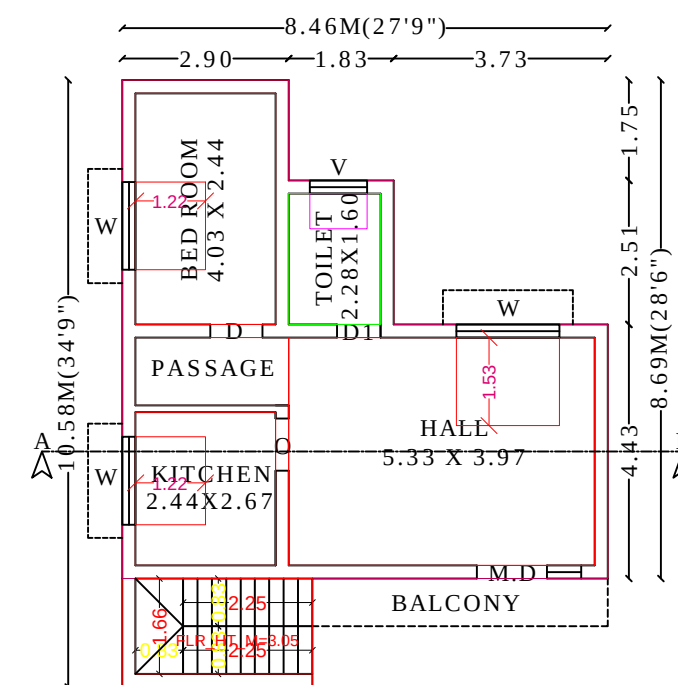
PRO.GROUND FLOOR PLAN (EAST FACING)
