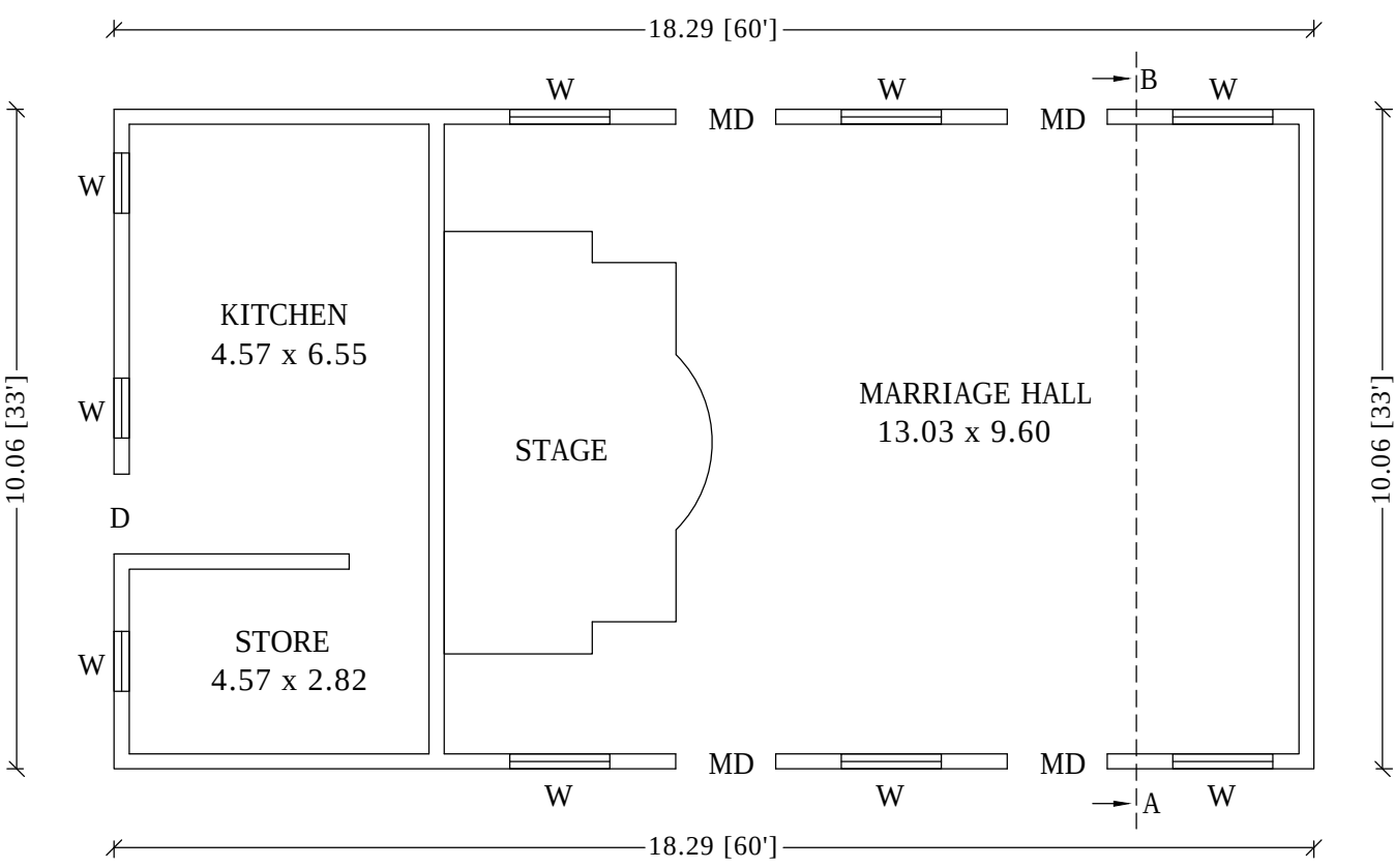
GROUND FLOOR PLAN ( MARRIAGE HALL )
