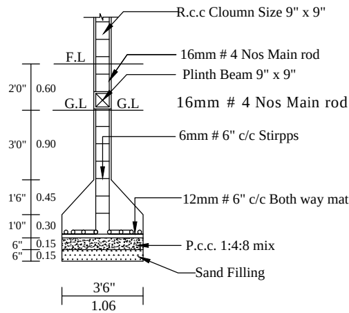
COLUMN DETIAL
