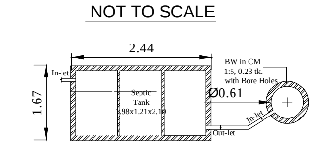
PLAN - SEPTIC TANK & SOAK PIT
