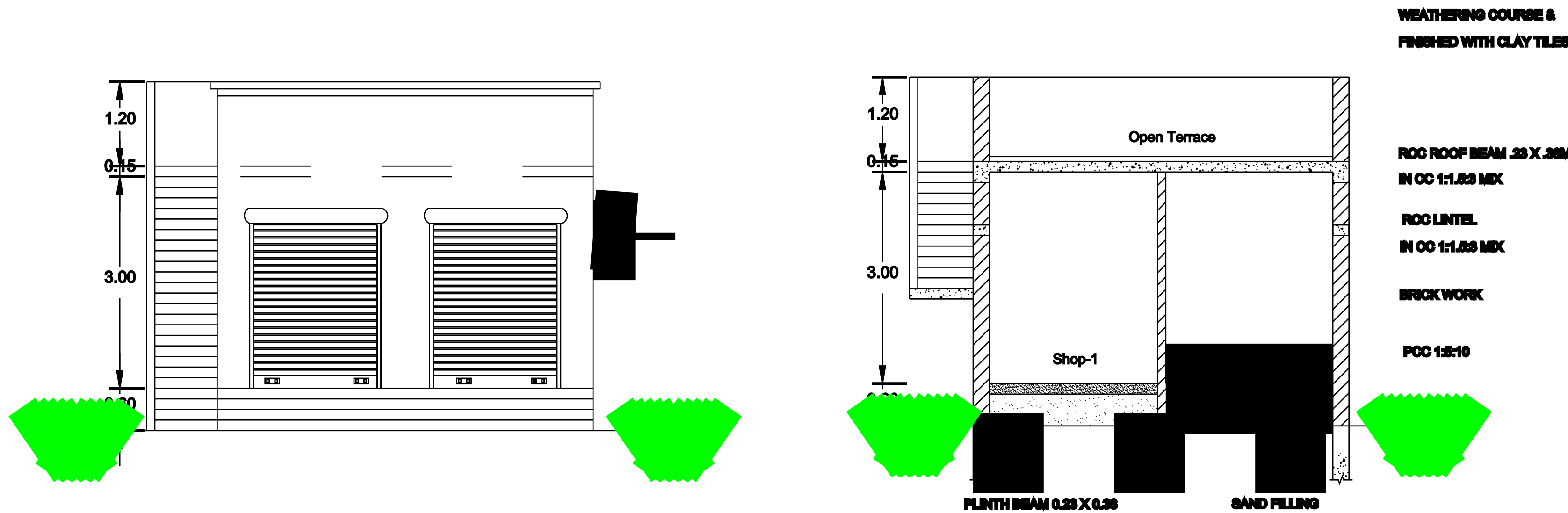
FRONT ELEVATION
