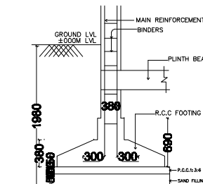
TYPICAL SECTION OF R.C.C COLUMN FOUNDATION
