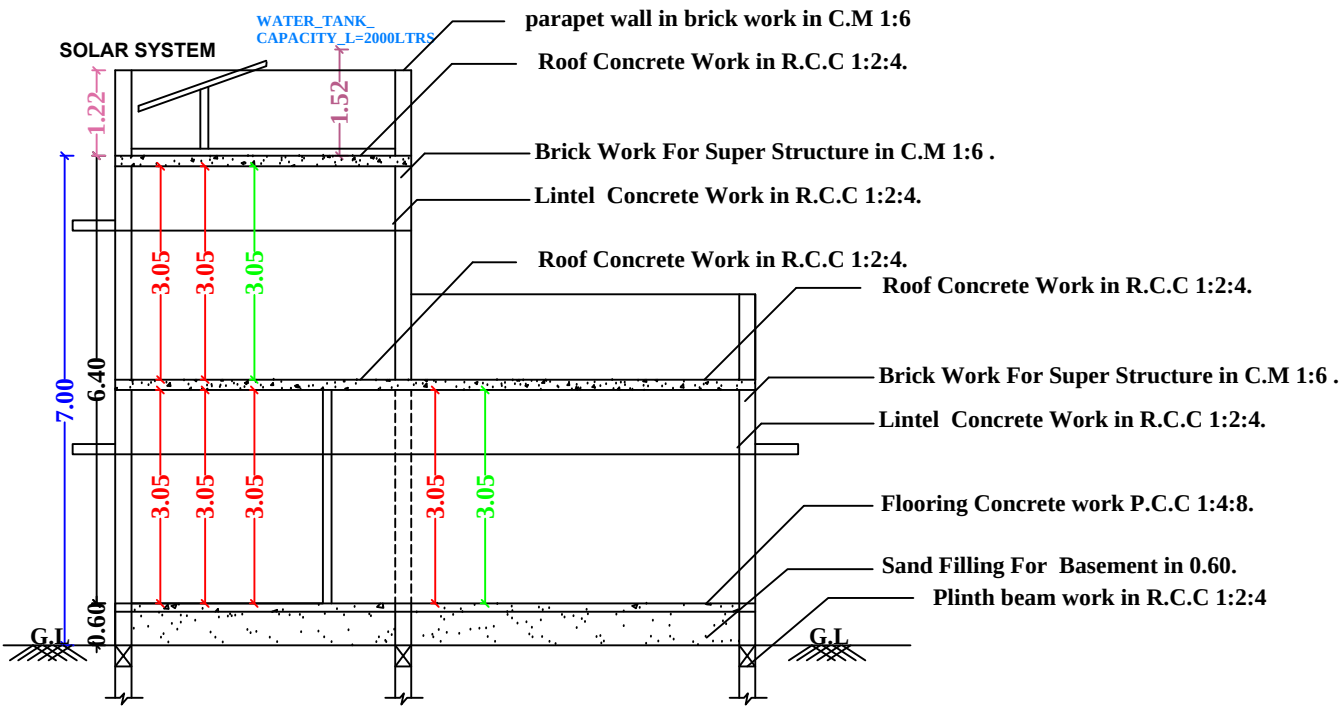
SECTION-AB
